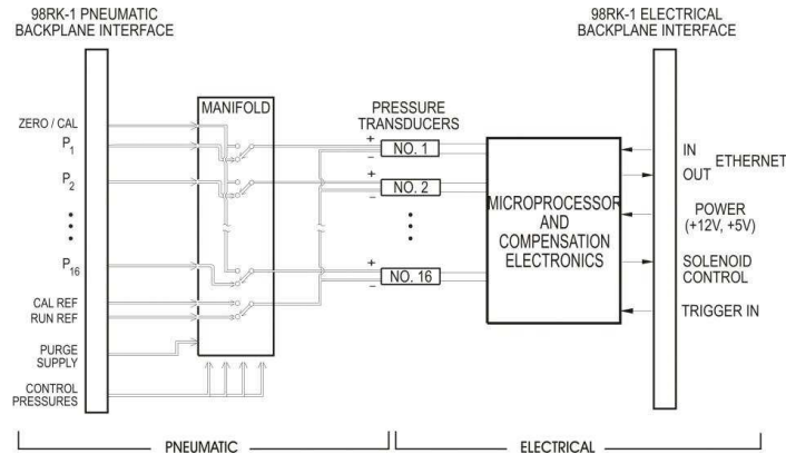
Pneumatic Intelligent Pressure Scanner Functional Diagram
