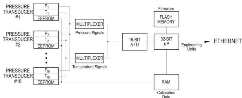
Digital Sensor Temperature Compensation Functional Diagram
