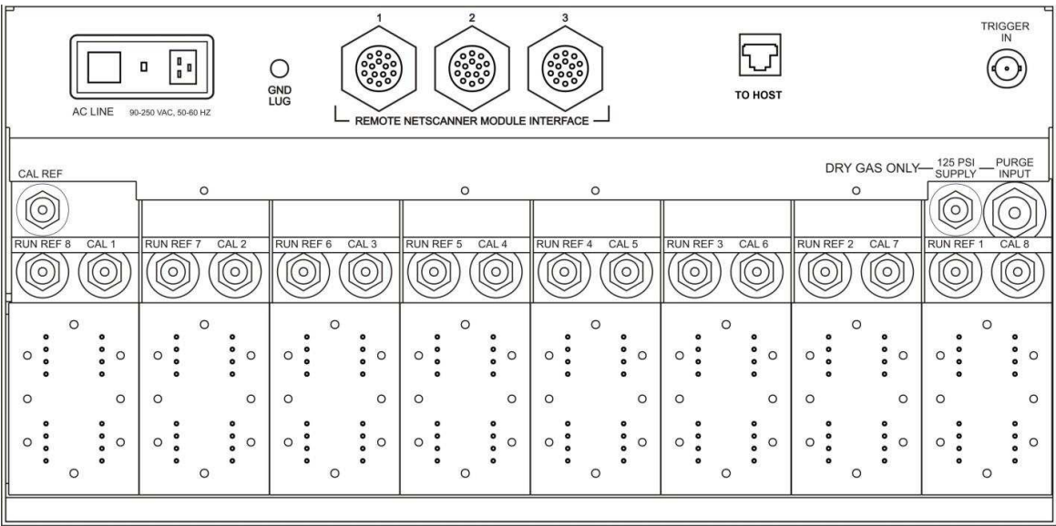
98RK-1 Scanner Interface Rack Rear Panel Layout
