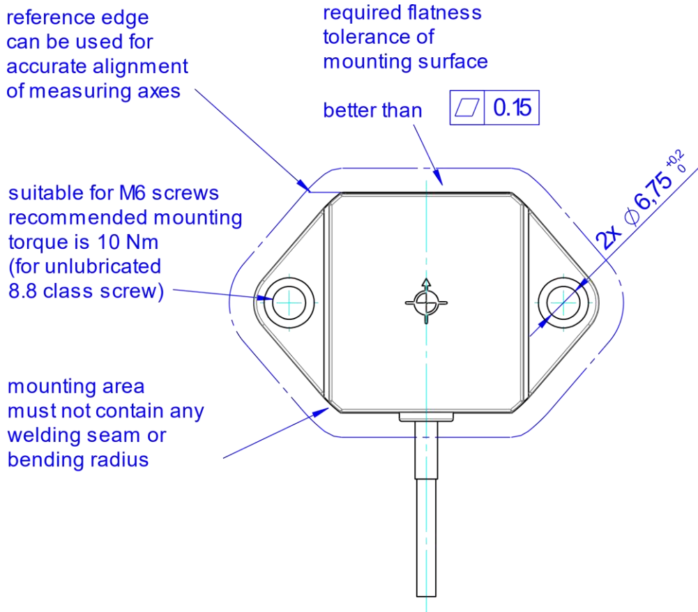
Figure 8: Mounting Detail
