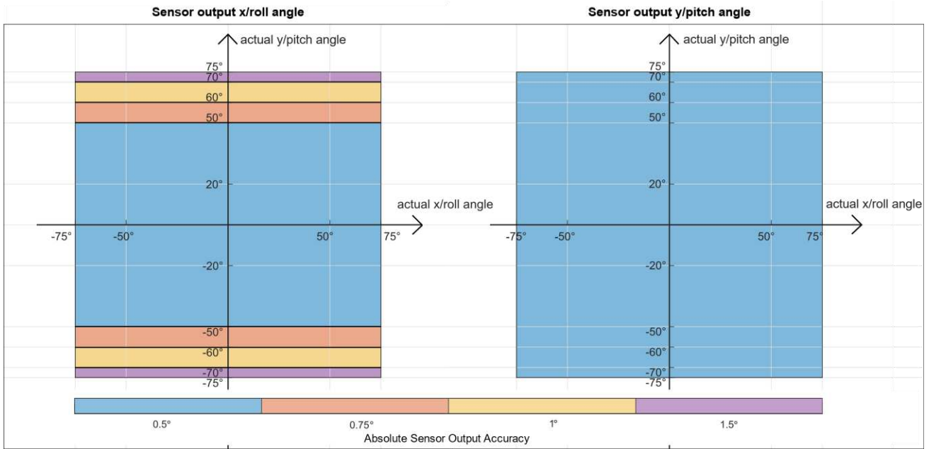
Figure 1: Definition of the absolute sensor output accuracy across the whole measurement range of \pm 75^\circ . Left: Sensor output x/roll angle. Interval-wise accuracy definition related to the actual y/pitch angle. Right: Sensor output y/pitch angle, constant accuracy throughout the whole measurement range.
