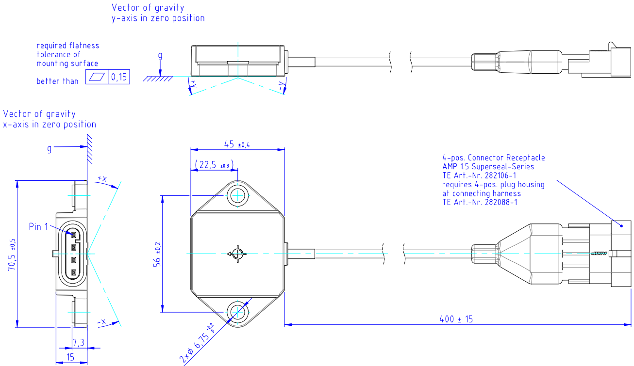
Figure 4: Dimensions
