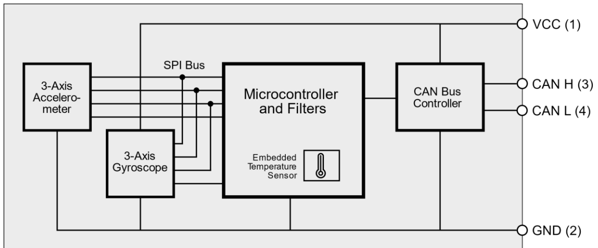
Figure 3: Block Diagram
