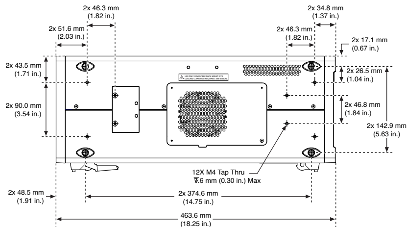
Figure 1. PXIe-1092 Chassis Dimensions (Side)
